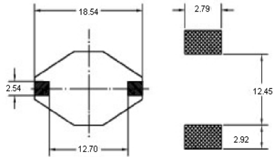
Pad Layout
